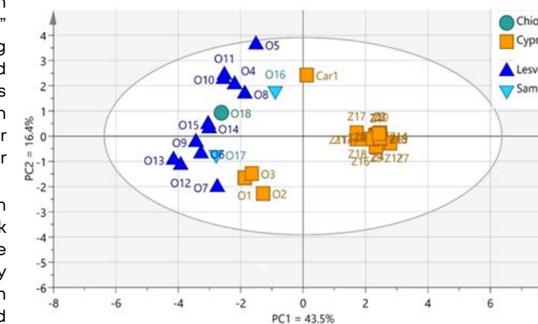
Scatter Plot for spirits from Cyprus and Greece based on their isotopic imprint: Z=zivania, Car=carob distillate, O=ouzo
